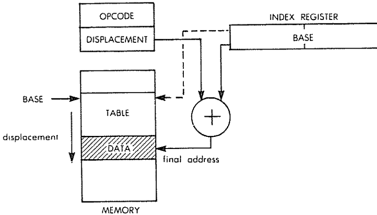
Fig. 5.2: Addressing (Pre-indexing)
