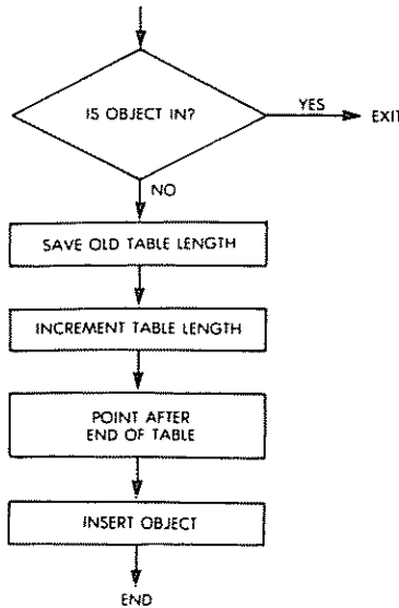
Fig. 9.13: Table Insertion Flowchart
